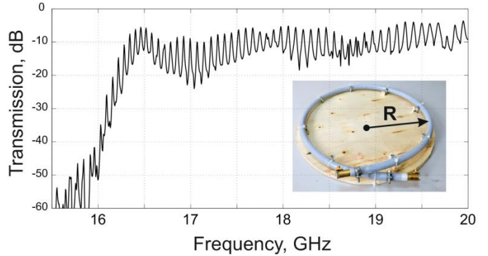
Fig. 5. Transmission trough bended metalized waveguide (Metalized polymer tube of 11 mm inner diameter, 1 meter length, 16 cm bending radius).
