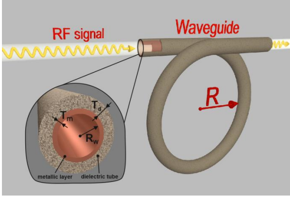
Fig. 1. Schematics of a metalized bendable dielectric tube for high frequency waveguiding applications.
