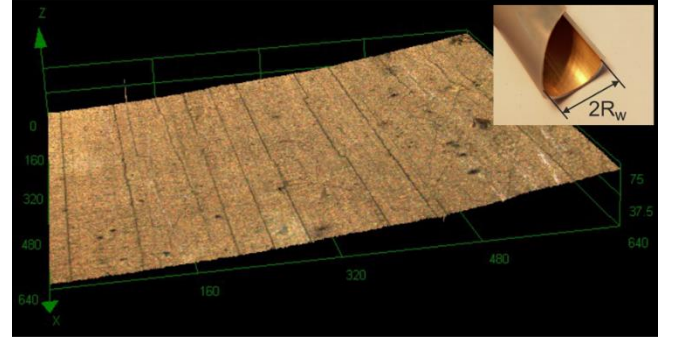
Fig. 2. Surface profile of 2.5 mm × 1 mm section of a metalized tube. (Inset) Photograph of the cut section of the tube.
